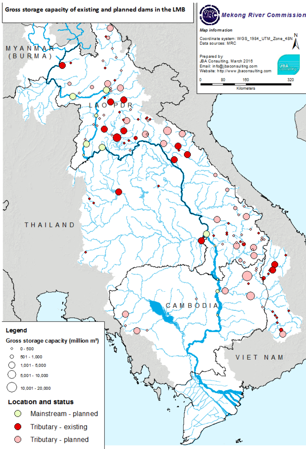
Figure 2.2. Hydropower projects (existing and planned in 2016) and their gross storage capacities.
