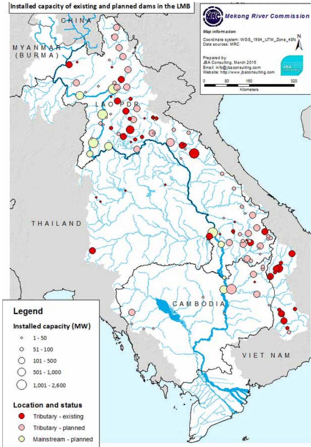
Figure 2.3. Hydropower projects (existing and planned in 2016) and their installed power capacities
