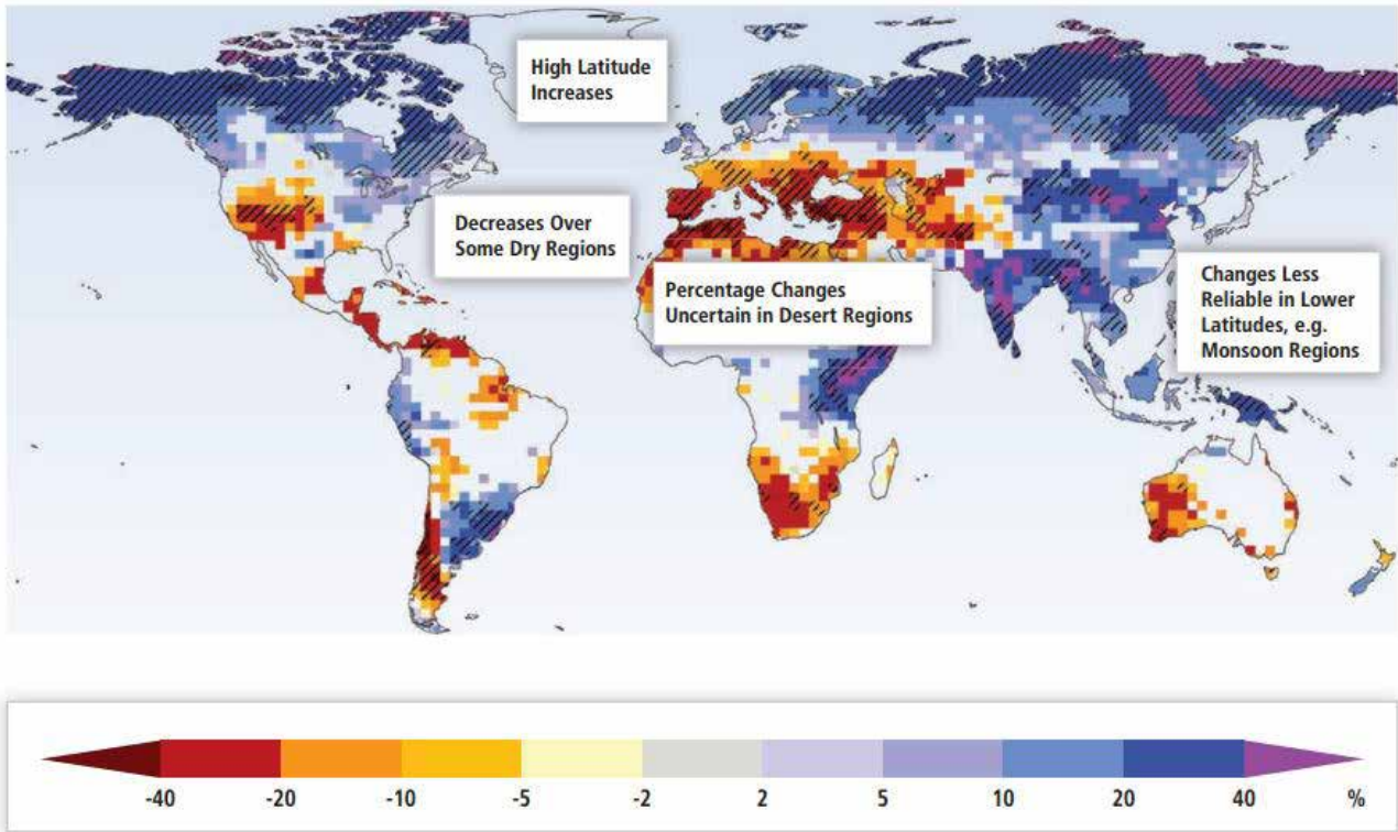
Figure 4.2 Global Distribution of Change in Runoff Median of 12 model projections for SRES A1B Scenario to 2099 as presented in IPCC SRREN report (2011)
