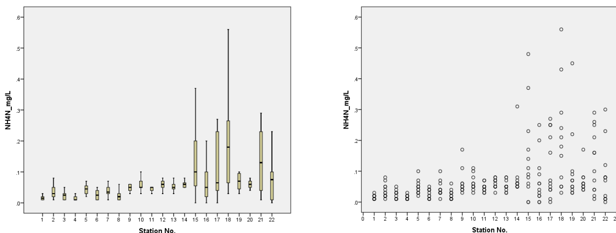
Figure 3.9 Spatial variation in ammonium concentrations in the Mekong River (1-17) and Bassac River (18-22) in 2017
