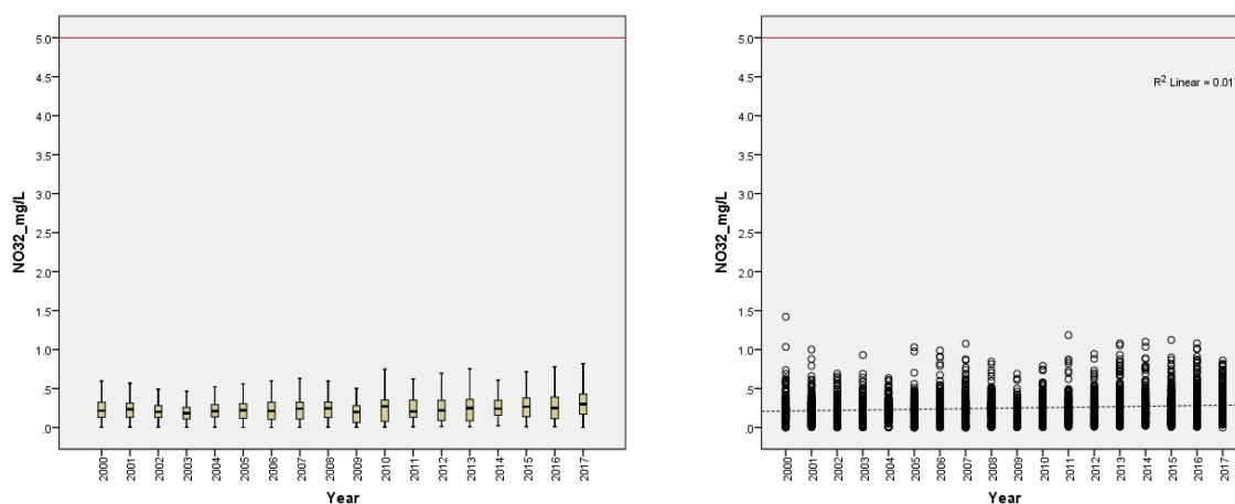
Figure 3.8 Temporal variation in nitrate-nitrite concentrations in the Mekong River as observed from 2000 to 2017 (the horizontal lines at 5.0 represent nitrate-nitrite limits of the MRC Water Quality Guidelines for the Protection of Human Health)
