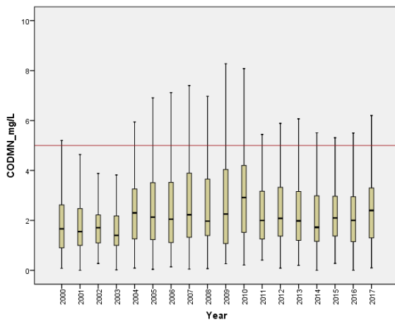
Figure 3.16 Temporal variation in COD (mg/L) in the Mekong River as recorded from 2000 to 2017 (the horizontal lines at 5.0 represent COD target value of the MRC Water Quality Guidelines for the Protection of Human Health)
