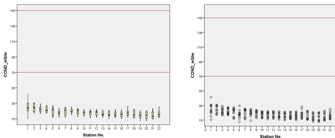
Figure 3.3 Spatial variation in Electrical Conductivity levels along the Mekong River (1-17) and Bassac River (18-22) as observed in 2017 (the horizontal lines at 70 and 150 represent lower and upper EC limits of the MRC Water Quality Guidelines for the Protection of Human Health)
