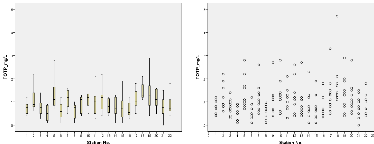
Figure 3.11 Spatial variation in total phosphorus concentrations in the Mekong River (1-17) and Bassac River (18-22) in 2017
