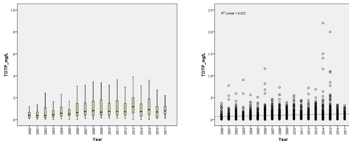
Figure 3.12 Temporal variation in total phosphorus concentrations in the Mekong River as observed from 2000 to 2017
