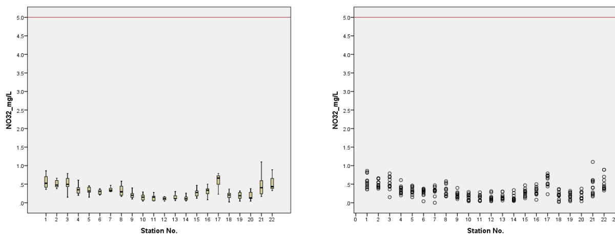
Figure 3.7 Spatial variation in nitrate-nitrite concentrations in the Mekong River (1-17) and Bassac River (18-22) in 2017 (the horizontal lines at 5.0 represent nitrate-nitrite limits of the MRC Water Quality Guidelines for the Protection of Human Health)
