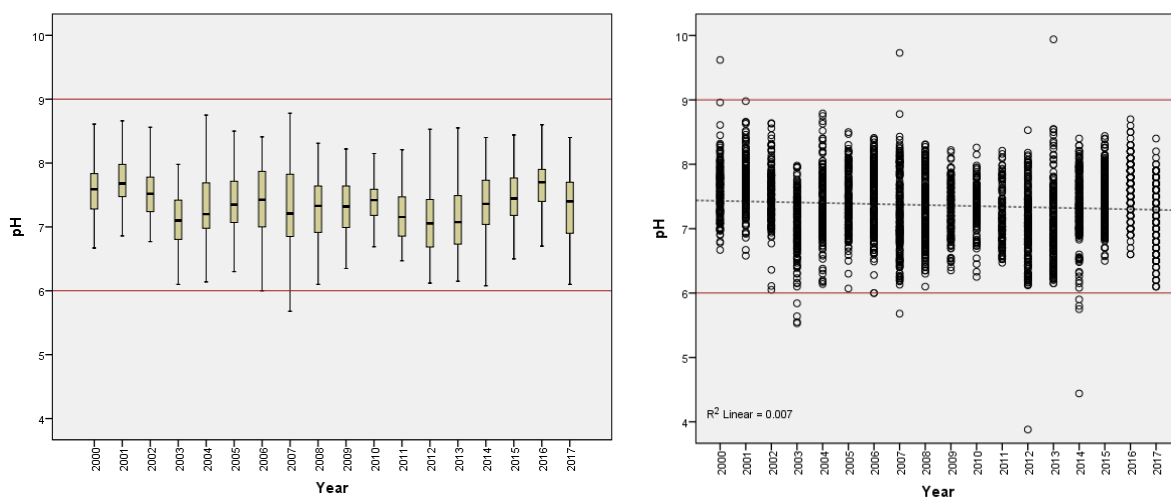
Figure 3.2 Temporal variation in pH levels in the Mekong River from 2000 - 2017 (the horizontal lines at 6.0 and 9.0 represent lower and upper pH limits of the MRC Water Quality Guidelines for the Protection of Aquatic Life and Protection of Human Health)
