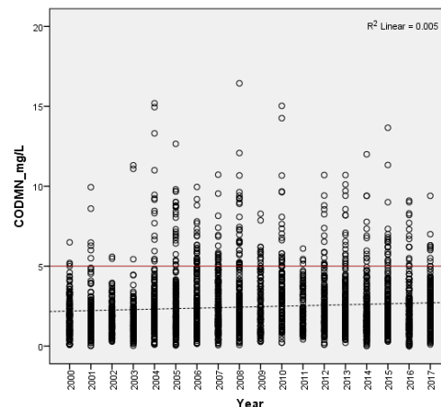
Figure 3.16 Temporal variation in COD (mg/L) in the Mekong River as recorded from 2000 to 2017 (the horizontal lines at 5.0 represent COD target value of the MRC Water Quality Guidelines for the Protection of Human Health)
