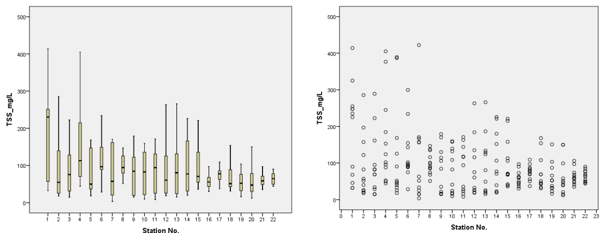
Figure 3.5 Spatial variation in TSS concentrations along the Mekong River (1-17) and Bassac River (18-22) as observed in 2017
