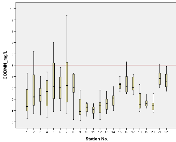
Figure 3.15 Spatial variation in COD (mg/L) at 22 stations along the Mekong (1-17) and Bassac (18-22) Rivers in 2017 (the horizontal lines at 5.0 represent COD target value of the MRC Water Quality Guidelines for the Protection of Human Health)
