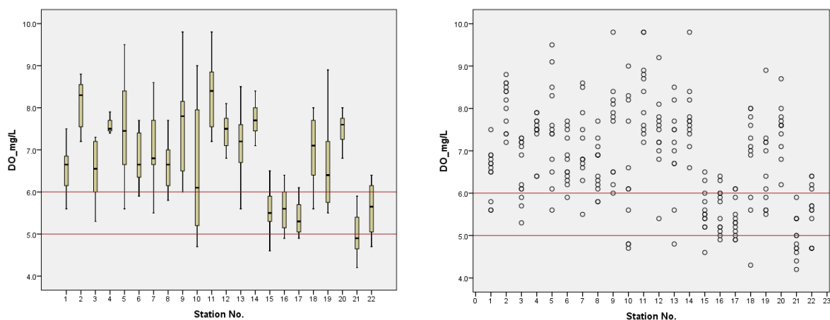
Figure 3.13 Spatial variation in dissolved oxygen (mg/L) at 22 stations along the Mekong (1-17) and Bassac (18-22) Rivers in 2017 (the horizontal lines at 5.0 and 6.0 represent DO target values of the MRC Water Quality Guidelines for the Protection of Human Health and Protection of Aquatic Life respectively)
