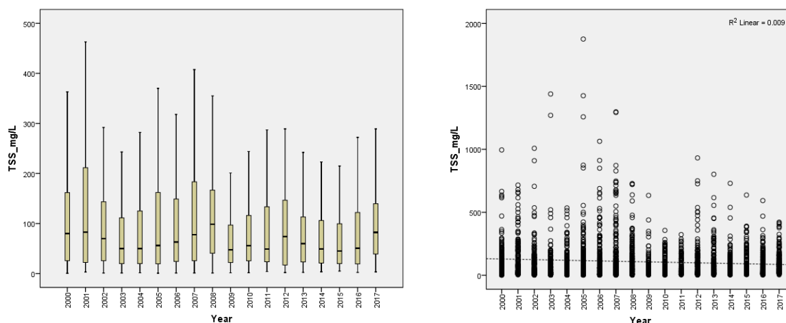
Figure 3.6 Temporal variation in TSS concentrations along the Mekong River as observed from 2000 to 2017
