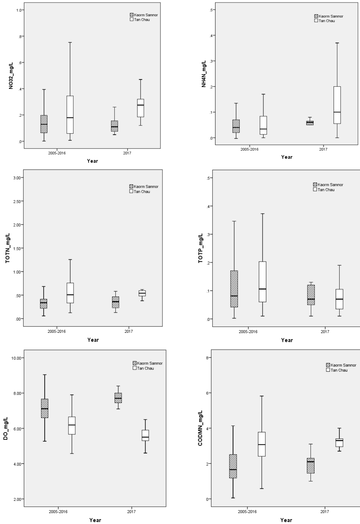
Figure 3.18 Comparisons of water quality data at Kaorm Samnor and Tan Chau
