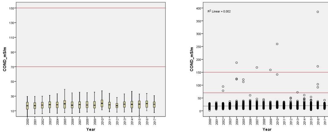
Figure 3.4 Temporal variation in Electrical Conductivity levels in the Mekong River as observed from 2000 to 2017 (the horizontal lines at 70 and 150 represent lower and upper EC limits of the MRC Water Quality Guidelines for the Protection of Human Health)
