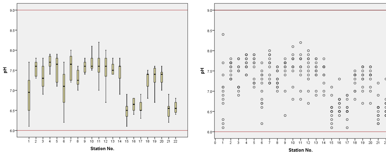
Figure 3.1 Spatial variation in pH levels along the Mekong River (Stations: 1-17) and Bassac River (Stations: 18-22) as observed in 2017 (the horizontal lines at 6.0 and 9.0 represent lower and upper pH limits of the MRC Water Quality Guidelines for the Protection of Aquatic Life and Protection of Human Health)
