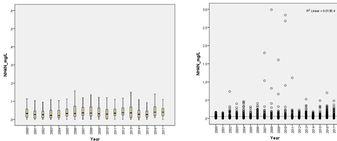
Figure 3.10 Temporal variation in ammonium concentrations in the Mekong River as observed from 2000 to 2017
