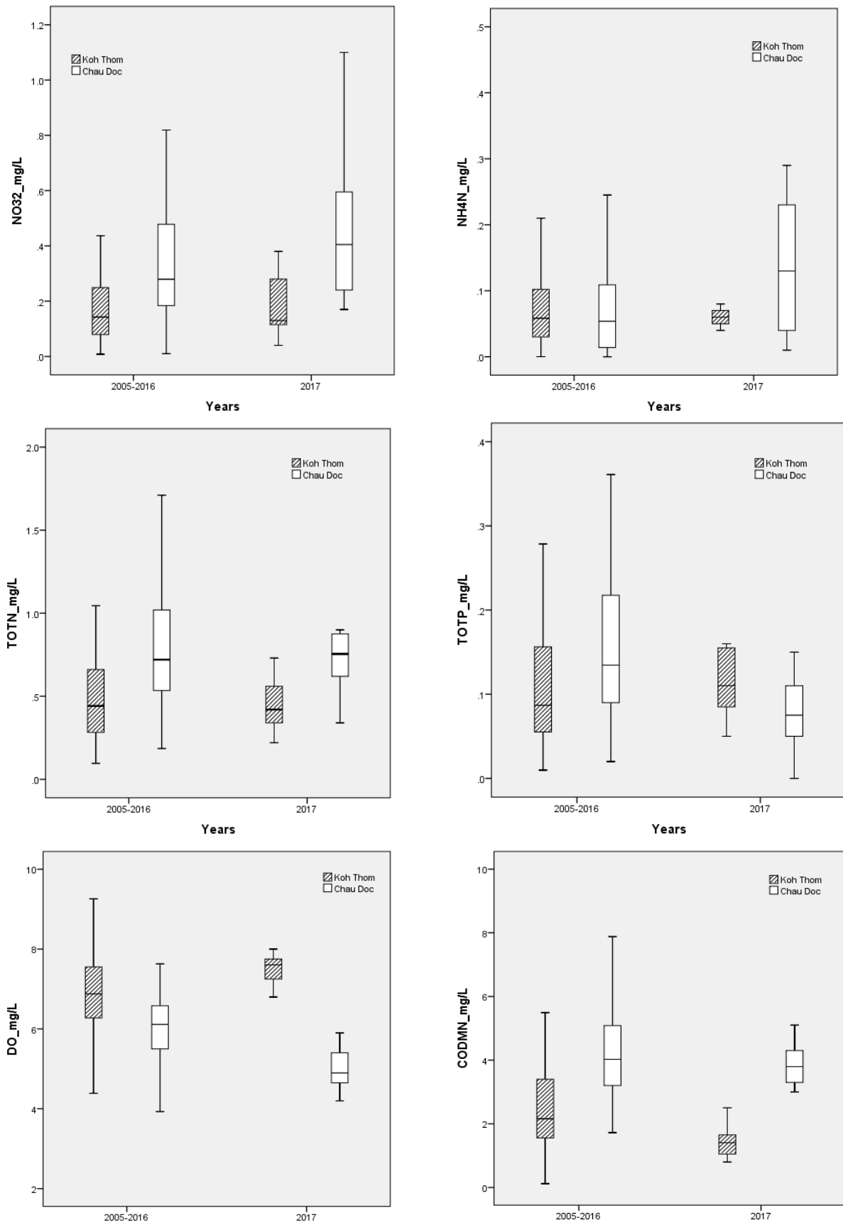
Figure 3.19 Comparisons of water quality data at Koh Thom and Chau Doc
