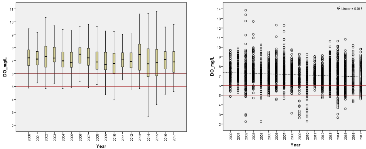
Figure 3.14 Temporal variation in dissolved oxygen (mg/L) in the Mekong River as recorded from 2000 to 2017 (the horizontal lines at 5.0 and 6.0 represent DO target values of the MRC Water Quality Guidelines for the Protection of Human Health and Protection of Aquatic Life respectively)
