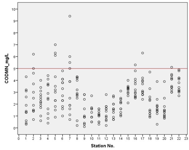
Figure 3.15 Spatial variation in COD (mg/L) at 22 stations along the Mekong (1-17) and Bassac (18-22) Rivers in 2017 (the horizontal lines at 5.0 represent COD target value of the MRC Water Quality Guidelines for the Protection of Human Health)
